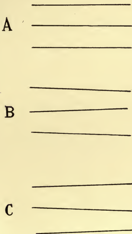
FIG. 176— Appearance presented by forms of heterophoria when a double prism, bases horizontal, is held before the right eye and the observer views a distant horizontal line. (A) Orthophoria; (B) tipping of the vertical axes inward; (C) tipping of the vertical axes outward.
